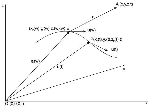
Fig. 1: A material point particle moving arbitrarily. As the material particle moves from point E(x_p(w), y_p(w), z_p(w), w) to point P(x_p(t), y_p(t), z_p(t), t) , the generalized photon moves from point E(x_p(w), y_p(w), z_p(w), w) to point A(x, y, z, t) .
